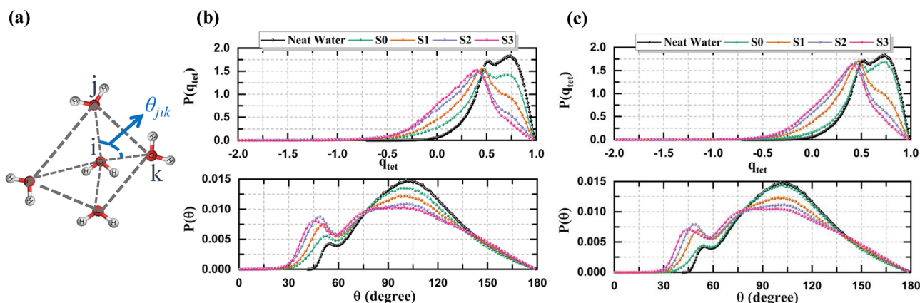
Fig. 9 (a) Schematic showing the tetrahedral geometry of water with the angle formed between the lines connecting the central water's oxygen ( i ) to the oxygens of its two nearest partners ( j , k ) of the four immediate water molecules. Probability distribution of the tetrahedral order parameter, P(q_{\text{tet}}) and angle subtended by two partners with the central water's Ow, P(\theta) for (b) solvation shell water and (c) bulk water molecules for all the systems studied. Probability distributions for P(q_{\text{tet}}) and P(\theta) obtained from the simulation of the neat water are also provided for comparison purposes represented by the black color.
