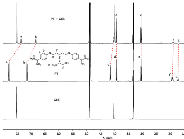
Fig. 17 1 H NMR spectra of C8S, pentamidine isethionate (PT) and host-guest complex – in the presence of some precipitate, recorded on an Agilent 400 MHz instrument at room temperature in CD 3 OD. c(C8S) = 4 mM, c(pentamidine) = 4 mM.
