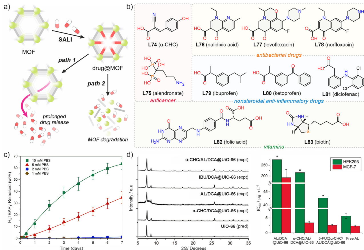
Fig. 9 (a) Scheme of the preparation of SALI-based drug delivery system (drug@MOF) and two possible pathways of drug release: path 1 based on slow decoordination of introduced molecules (reverse-SALI) and path 2 where MOF degradation leads to more rapid drug release. 169 (b) Examples of bioactive molecules introduced into MOF via SALI technique; \alpha -CHC = \alpha -cyano-4-hydroxycinnamic acid. (c) Stability in different concentrations of PBS of representative Zr-MOF (NU-1000) studied as drug delivery system. 169 Reprinted from ref. 169 with permission. Copyright 2018 Elsevier. (d) Powder X-ray diffraction (PXRD) patterns of drug-loaded UiO-66 (left) and comparison of IC 50 values of drug-loaded UiO-66 compared with free alendronate (AL) against HEK293 and MCF-7 cell lines. 45 Figure adapted from ref. 45 with permission. Copyright 2020 John Wiley and Sons.
