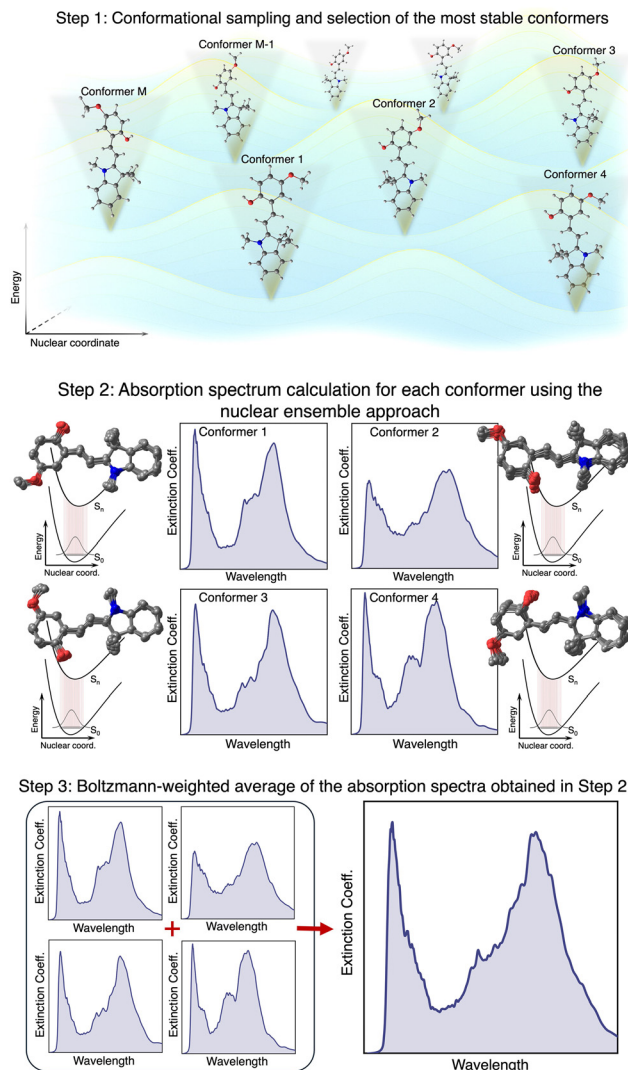
Fig. 1 Schematic of the computational protocol proposed to calculate absorption spectra of complex molecules, illustrated using \text{MCH}^+ . Hydrogen atoms are omitted in step 2 for clarity.
