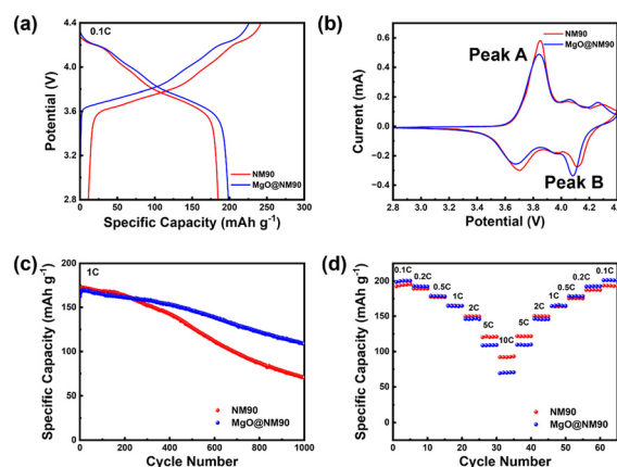
Fig. 2 (a) The initial charge and discharge curves of NM90 and MgO@NM90 at 0.1C rate ( 1\text{C} = 180 \text{mAh g}^{-1} ). (b) CV curves of NM90 and MgO@NM90 between 2.8 and 4.4 V (scan rate: 0.1 \text{mV s}^{-1} ). (c) Cycling performance of NM90 and MgO@NM90 at 1C. (d) Rate capability of the two samples from 0.1C to 10C between 2.8 and 4.4 V.
