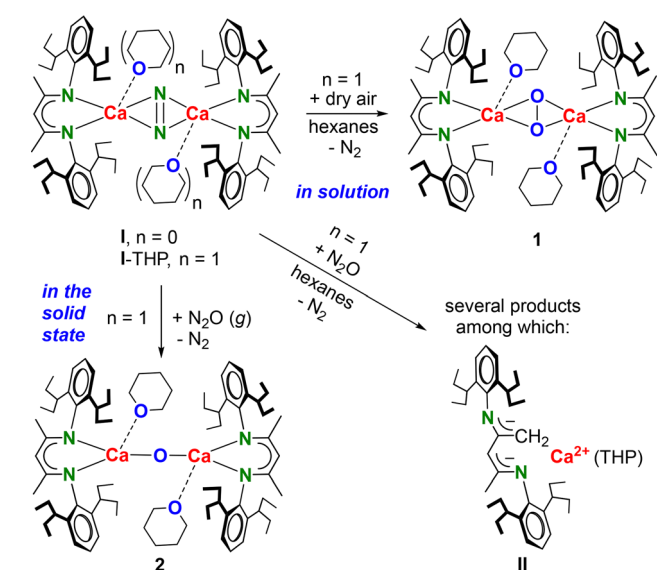
Scheme 2 Synthesis of low-coordinate Ca peroxide ( 1 ) and Ca oxide ( 2 ) complexes.
