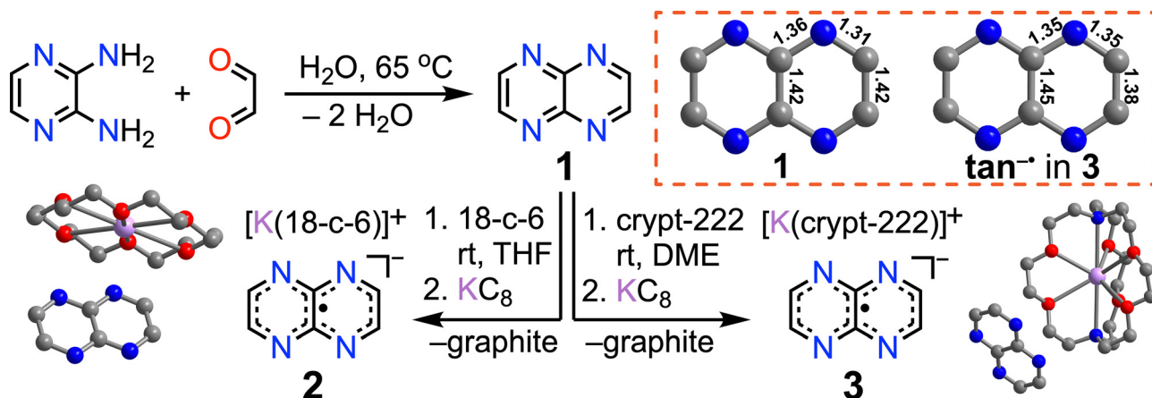
Fig. 1 Synthesis of tan, 1 , [K(18-c-6)]tan•, 2 , and [K(crypt-222)]tan•, 3 , along molecular structures of 2 (bottom left) and 3 (bottom right). Box with the dashed outline shows the molecular structures of neutral tan, 1 , and tan• in 3 . Distances (Å) are rounded up for clarity and full values can be found in the main text; both are planar, see Fig. S12 (ESI†). For all crystal structures: grey, blue, red and purple spheres represent C, N, O and K atoms, respectively. H atoms and co-crystallised solvent molecules have been omitted for clarity.
