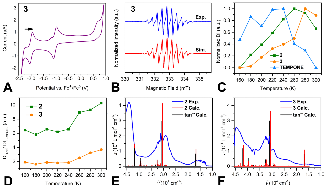
Fig. 2 (A) Cyclic voltammogram of [K(\text{crypt-222})]\text{tan}^\bullet , 3 , vs. Fc. (B) X-band cw-EPR spectrum of 3 . The experimental spectrum was collected at 300 K (blue trace) and the simulation is shown in red trace. (C) Temperature dependence of normalized EPR double intensity (DI) values of 2 (green squares), 3 (orange circles), and the standard TEMPONE (light blue triangles). (D) Corrected EPR DI values of 2 (green squares) and 3 (orange circles) obtained by dividing the DI of \text{tan}^\bullet by DI of TEMPONE at each respective temperature. UV-Vis spectra of (E) 20 \mu\text{M} solution of 2 and (F) 15 \mu\text{M} solution of 3 . Both spectra (blue trace) were collected in THF from 220 nm to 1000 nm. The red vertical lines correspond to predicted TD-DFT transitions. Black vertical lines exhibit the predicted transitions for the \text{tan}^\bullet fragment.
