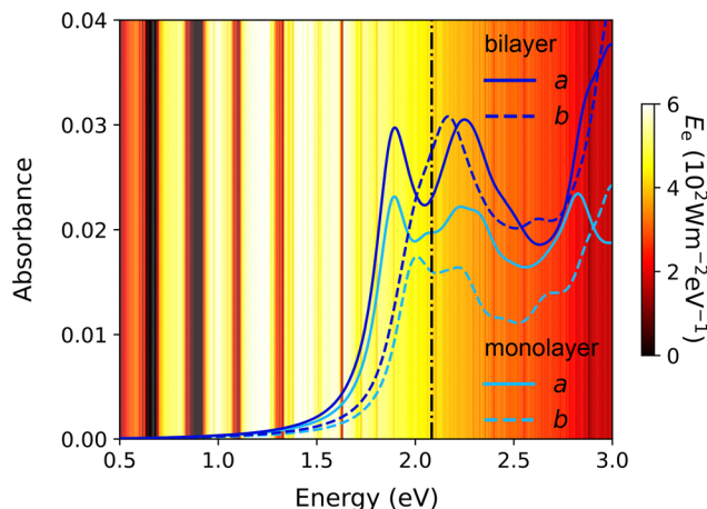
Fig. 11 Optical absorbance of monolayer and bilayer fullerene networks for both a and b polarisations. The black vertical dash-dot lines represent the direct band gaps from independent-particle approximations in the absence of excitons. The background shows the global total spectral irradiance E_e from the Sun. 93
