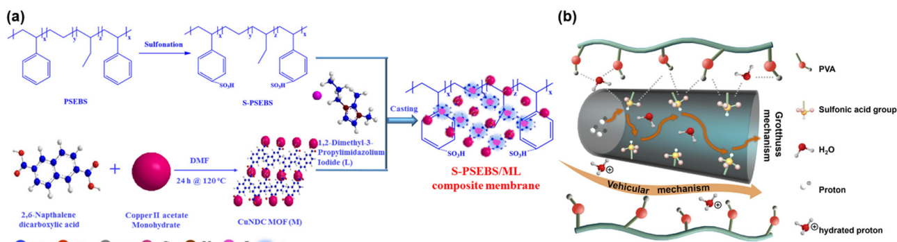
Fig. 9 (a) Schematic representation for preparation of S-PSEBS/ML composite membrane. Reproduced with permission from ref. 83, Copyright 2022, American Chemical Society. (b) The possible proton transport pathways of CL-PVA/Cu-MOF-15. Reproduced with permission from ref. 84, Copyright 2023, Elsevier.
