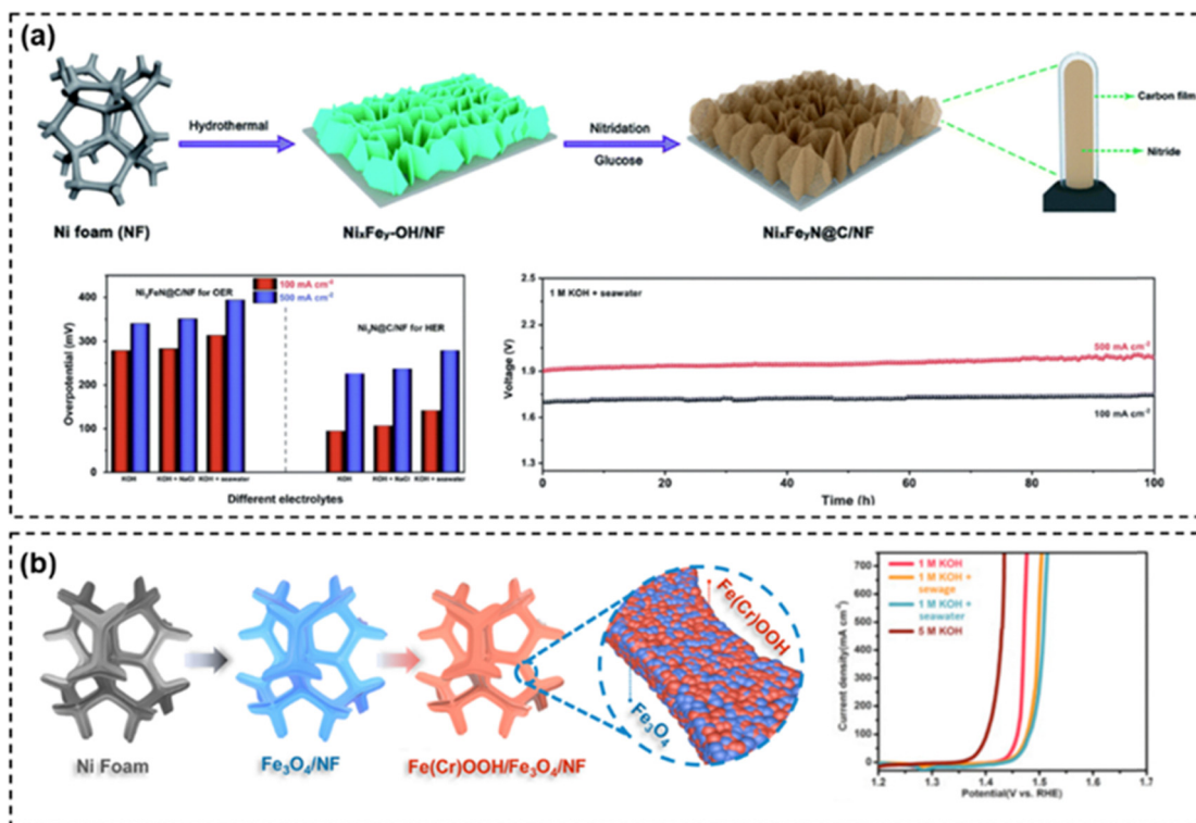
Fig. 15 Seawater-splitting OER electrocatalysts: Schematic of the preparation of (a) Ni x Fe y N@C/NF with a comparison of the overpotentials for HER and OER at 100 mA cm -2 and 500 mA cm -2 in different electrolytes and durability tests of the electrolyzer at 100 mA cm -2 and 500 mA cm -2 in 1 M KOH and alkaline seawater in 1 M KOH 223 and (b) Fe(Cr)OOH/Fe 3 O 4 /NF with LSV curves for OER at high current densities measured in different electrolytes. 218 Reproduced with permissions from ref. 223, Copyright 2021 Royal Society of Chemistry, ref. 218, Copyright 2022 Elsevier.
