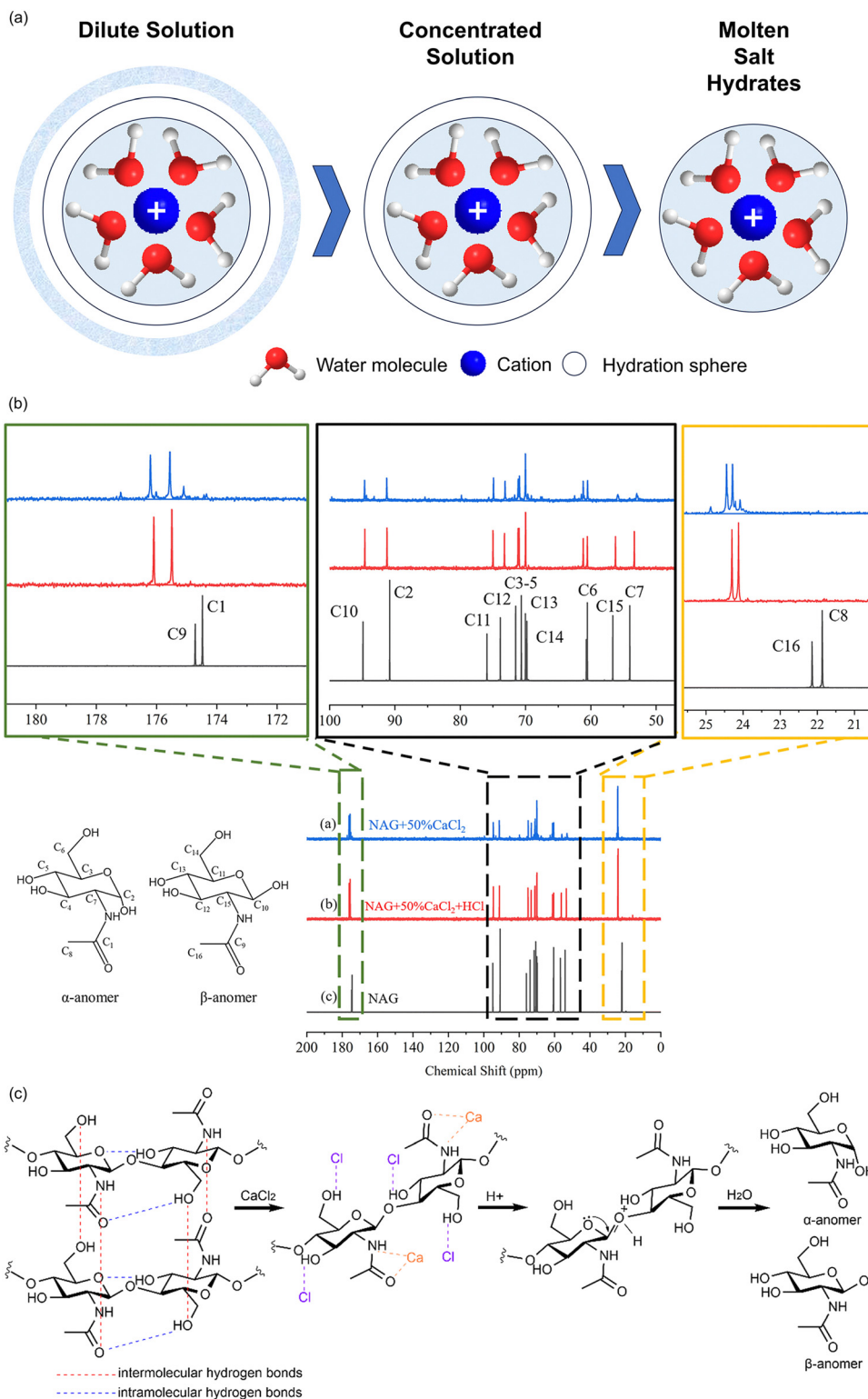
Fig. 7 (a) Graphical depiction of salt solutions with varying salt concentrations. The interaction between chitin and Ca 2+ cations and Cl - anions. (b) 13 C NMR spectra of NAG and CaCl 2 . (c) The proposed interaction mode between chitin and Ca 2+ cations and Cl - anions. Reproduced from ref. 110 with permission from The Royal Society of Chemistry, copyright 2023.
