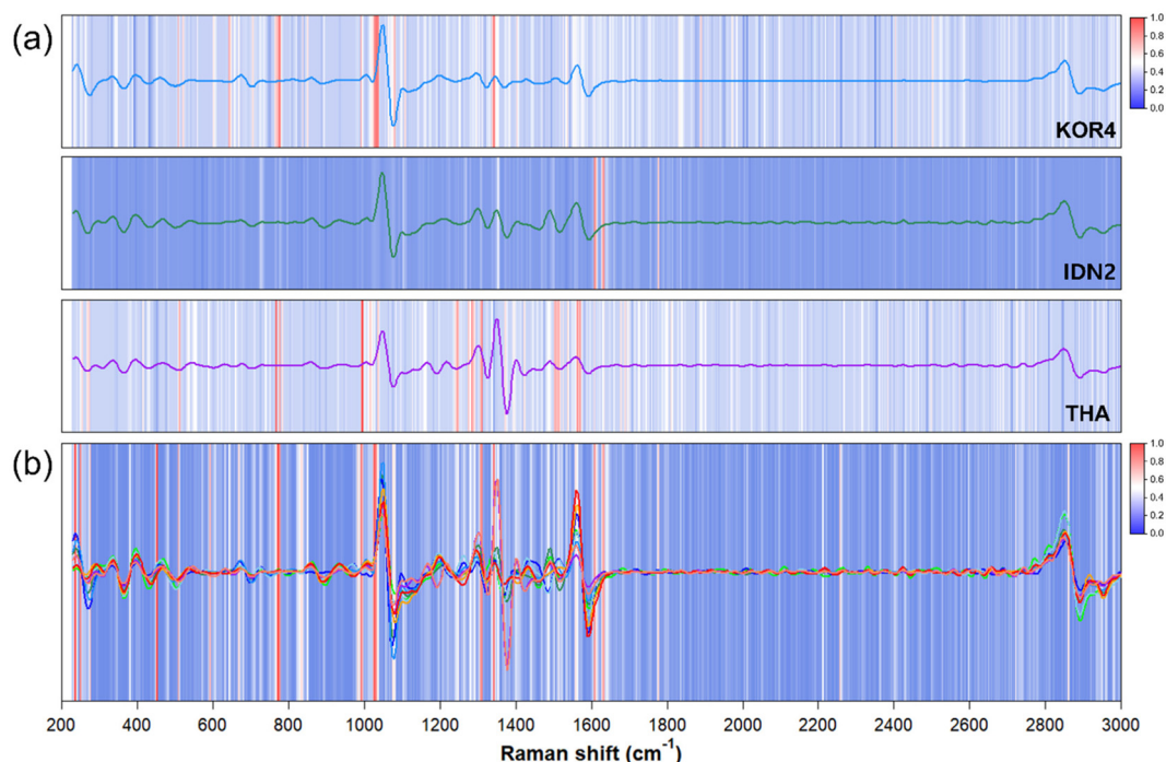
Fig. 6 Raman spectral-feature importance analysis of the RF model when classifying document paper samples. Spectral feature importance of the KOR4, IDN2, and THA products (a) and entire data classes (b). Red indicates higher importance, while blue indicates lower importance.
