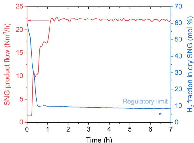
Fig. 2 Productivity and H_2 fraction in SNG at the reactor outlet at the start-up of the biogas methanation plant (experimental conditions: 8 bar, H_2 : CO_2 = 4.15 , cooling setpoint = 230\text{ }^{\circ}\text{C} ). The CO_2 conversion is 100% in the entire time interval considered and no other products than methane were observed.
