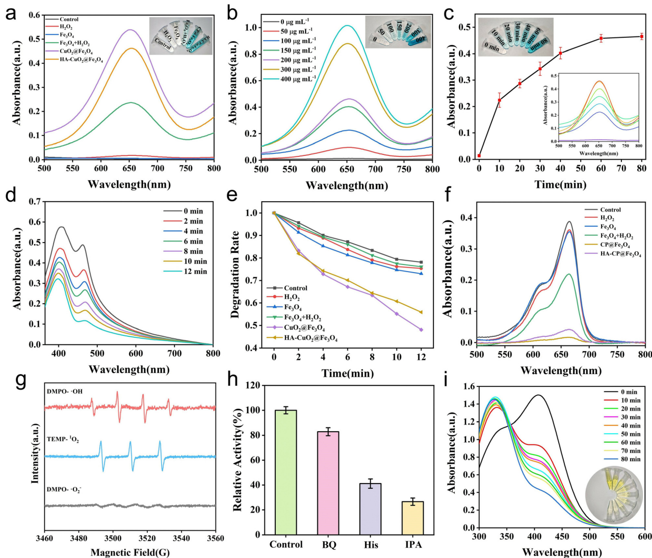
Fig. 3 (a) Confirmation of \bullet\text{OH} radicals generated by Fenton-like reaction in different groups ( 200 \mu\text{g mL}^{-1} ) using TMB assay. Studying Fenton activity of HA-CP@ \text{Fe}_3\text{O}_4 by varying (b) concentrations and (c) time ( 200 \mu\text{g mL}^{-1} ). (d) Absorption spectra of DPBF solution with HA-CP@ \text{Fe}_3\text{O}_4 ( 200 \mu\text{g mL}^{-1} ) at increasing time intervals. (e) Comparison of the degradation rates of DPBF over time in different experimental groups ( 200 \mu\text{g mL}^{-1} ). (f) Absorption spectra of MB after treatment with different experimental groups ( 200 \mu\text{g mL}^{-1} ). (g) ESR spin-trapping spectra of HA-CP@ \text{Fe}_3\text{O}_4 for the detection of \text{DMPO}-\bullet\text{OH} , \text{DMPO}-\bullet\text{O}_2^- , and \text{TEMP}-^1\text{O}_2 . (h) Inhibition of TMB oxidation by IPA, BQ, and His in the presence of HA-CP@ \text{Fe}_3\text{O}_4 . (i) Time-dependent depletion of GSH by HA-CP@ \text{Fe}_3\text{O}_4 ( 200 \mu\text{g mL}^{-1} ).
