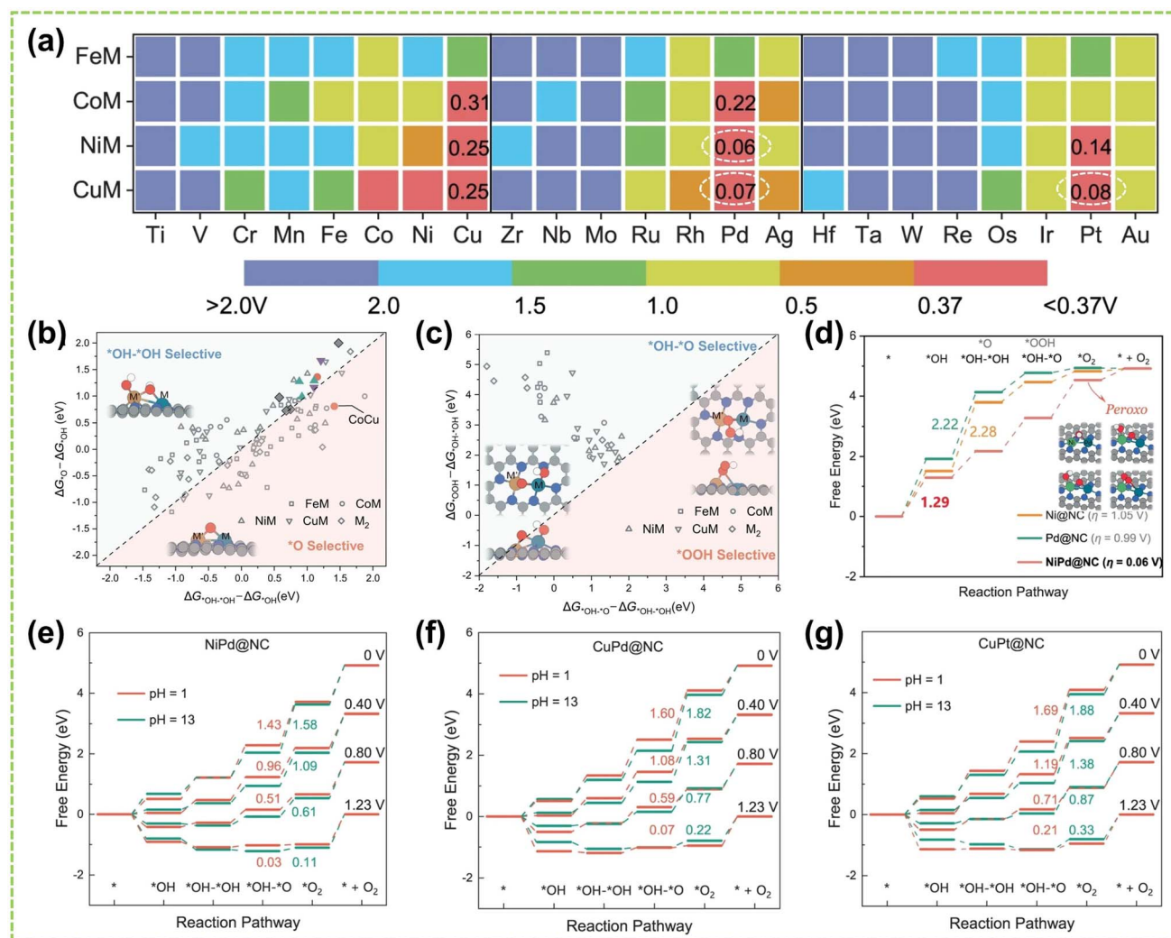
Fig. 19 The OER performance of DACs in all pH conditions. (a) Activity map. The computed overpotential of the FeM, CoM, NiM, and CuM dimers on M'M@NC . (b) \Delta G of \text{*OH} toward \text{*OH} \rightarrow \text{*OH} \rightarrow \text{*OH} \rightarrow \text{*O} + \text{H}^+ + \text{e}^- . Data points screened for high-performance homo- and hetero-nuclear catalysts are colored. (c) \Delta G of \text{*OH} \rightarrow \text{*OH} \rightarrow \text{*OH} \rightarrow \text{*O} + \text{H}^+ + \text{e}^- versus \text{*OH} \rightarrow \text{*OH} \rightarrow \text{*OH} \rightarrow \text{*OOH} + \text{H}^+ + \text{e}^- . Insets: the schematic configuration of the different intermediates adsorbed on M'M@NC . The white, red, gray, and blue spheres in the atomic models represent H, O, C, and N atoms, respectively. (d) Free energy diagrams of NiPd@NC and the respective corresponding SACs for OER. Inset: the optimized configurations of oxygenated intermediates represented as NiPd@NC. Free energy diagrams of (e) NiPd@NC, (f) CuPd@NC, and (g) CuPt@NC at different potentials with pH = 1 and 13 and the corresponding \Delta G_{\text{OH}} - \Delta G_{\text{OH}} \rightarrow \text{*O}_2 are labeled 89 (reproduced with permission from ref. 89 copyright 2023, Springer Nature).
