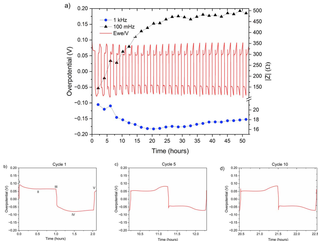
Fig. 7 (a) Left Y axis: a voltage trace ( E vs. t ) of successive galvanostatic cycling of a total of 0.5 \text{ mA h cm}^{-2} of zinc in a symmetric cell with 1 M \text{ZnSO}_4 aqueous electrolyte and a Celgard 3501 polymer separator. Constant current density 0.5 \text{ mA cm}^{-2} at 1C (plating and stripping 0.5 \text{ mA h cm}^{-2} , which is equivalent to 1.2 \text{ mg cm}^{-2} zinc). Right Y axis: impedance modulus at 0.1 Hz (black), 1 kHz (blue). (b)–(d) Magnification of selected voltage traces ( E vs. t ) of successive galvanostatic cycling of a total of 0.5 \text{ mA h cm}^{-2} of zinc in 1 M \text{ZnSO}_4 aqueous electrolyte. Cycles 1 (b), 5 (c), and 10 (d) are presented. Characteristic peaks and processes are labelled, following the assignments made by Dasgupta et al. 34
