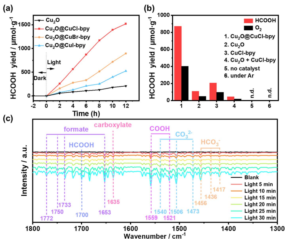
Fig. 4 (a) The yield of \text{HCOOH} as a function of the time of visible light illumination over \text{Cu}_2\text{O} and \text{Cu}_2\text{O}@ \text{CuX-bpy} . (b) The yield of \text{HCOOH} produced with different catalyst and reaction conditions after 6 h of visible light illumination. (c) In situ FTIR spectra for the simulated photo-driven \text{CO}_2 reduction process over \text{Cu}_2\text{O}@ \text{CuCl-bpy} .
