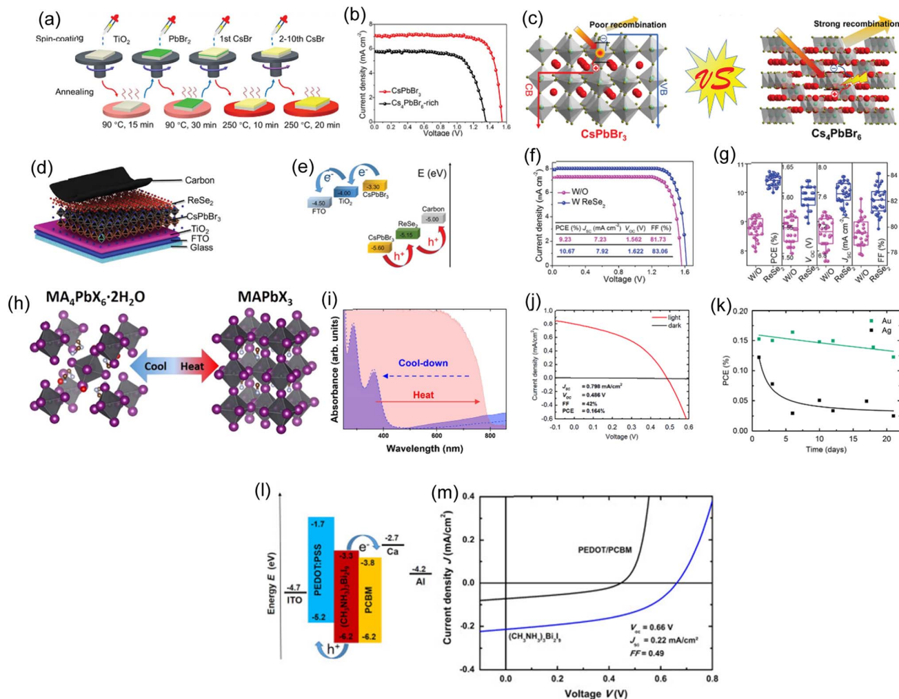
Fig. 2 (a) Schematic of the multi-step production method. (b) The J-V characteristics \text{CsPbBr}_3 based PSCs with and without \text{Cs}_4\text{PbBr}_6 . (c) The process by which carrier recombination was induced by \text{Cs}_4\text{PbBr}_6 . (d) All-inorganic \text{CsPbBr}_3 PSC with a \text{ReSe}_2 -tailored structure. (e) Energy level of the all-inorganic, \text{ReSe}_2 -tailored \text{CsPbBr}_3 PSC. (f) J-V curves. (g) Statistics of the PVs of different PSCs with and without \text{ReSe}_2 . (a)–(g) Reproduced with permission. 60 Copyright 2022, Wiley. (h) In the top left corner is the crystal structure of \text{MA}_4\text{PbI}_6 \cdot 2\text{H}_2\text{O} , and in the top right corner is \text{MAPbI}_3 . (i) Images illustrate the optical absorption of a pure sample of methylammonium lead iodide (blue), after thermal annealing at 100^\circ\text{C} (red), and after cooling to ambient temperature (blue dashes). (h) and (i) Reproduced with permission. 61 2021, ACS. (j) J-V characteristics. (k) The stability of MABI devices with Ag and Au top contacts is plotted as a PCE with time. (j) and (k) Reproduced with permission. 63 Copyright 2017, RSC. (l) Numbers in the energy level diagram are given in relation to the vacuum. (m) J-V curves for devices with a (\text{CH}_3\text{NH}_3)_3\text{Bi}_2\text{I}_9 absorber (blue) and a reference cell without an absorber (black) under illumination. (l) and (m) Reproduced with permission. 63 Copyright 2016, Elsevier.
