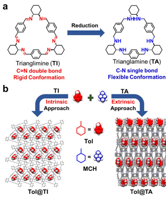
Fig. 1 (a) Chemical structures of TI and TA and their transformation. (b) Schematic illustration of the intrinsic and extrinsic capture approaches of Tol from the mixture of Tol/MCH by TI and TA.
