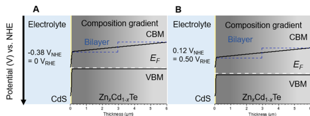
Fig. 8 Expected band diagrams for the cases of the bilayer structure and the composition gradient structure of ZnTe and CdTe at (A) 0 \text{ V}_{\text{RHE}} and (B) 0.5 \text{ V}_{\text{RHE}} .
