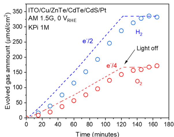
Fig. 10 Hydrogen and oxygen evolution from the ITO/Cu/ZnTe/CdTe/CdS/Pt (RTA) photocathode under simulated sunlight in a three-electrode configuration with an applied potential of 0 \text{ V}_{\text{RHE}} . The expected amounts of hydrogen and oxygen (denoted as e^-/2 and e^-/4 , respectively) as calculated from the observed photocurrent are shown as dashed lines. A 1 M aqueous KPi solution with pH adjusted to 6.5 with KOH was used as the electrolyte.
