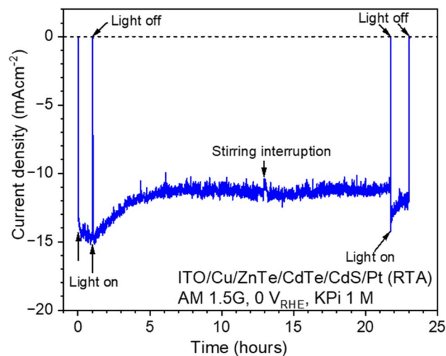
Fig. 9 Time course of the photocurrent generated by an ITO/Cu/ZnTe/CdTe/CdS/Pt photocathode at 0 \text{ V}_{\text{RHE}} under simulated sunlight in 1 M KPi aqueous solution under 400 rpm stirring.
