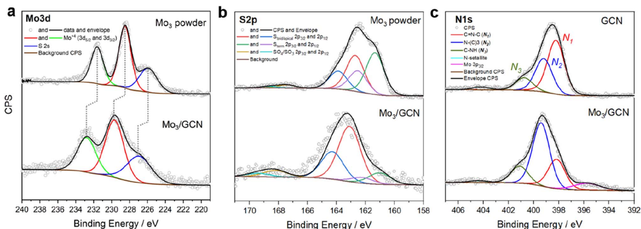
Fig. 3 XPS spectra of the \text{Mo}_3/\text{GCN} cluster. The [\text{Mo}_3\text{S}_{13}]^{2-} clusters before ( \text{Mo}_3 powder) and after ( \text{Mo}_3/\text{GCN} ) attachment to the GCN surface, (a) Mo 3d, (b) S 2p, and (c) N 1s ( \text{N}_1 : pyridinic nitrogen; \text{N}_2 : quaternary nitrogen; \text{N}_3 : secondary amine), with corresponding fits.
