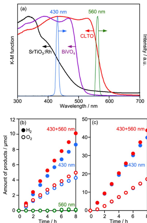
Fig. 10 (a) UV-vis spectra of CLTO, BiVO_4 and SrTiO_3 :Rh reduced by H_2 , and spectra of monochromatic light at 430 and 560 nm. Z-WS in 0.1 mM Co(bpy)_3SO_4 by (b) Cr_2O_3 /Ru/CLTO- BiVO_4 and (c) Ru/ SrTiO_3 :Rh- BiVO_4 systems under different irradiation conditions.
