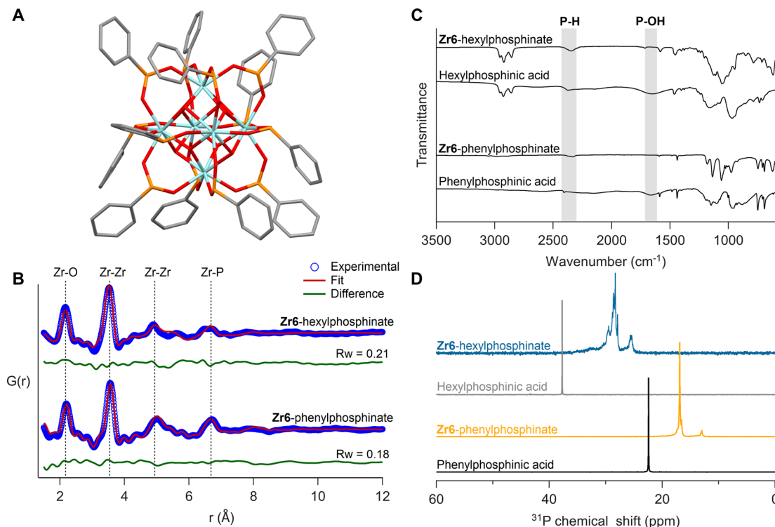
Fig. 6 (A) Crystal structure of Zr6 -phenylphosphinate cluster – Zr 6 O 8 H 4 (O 2 PHPh) 12 . Cyan atoms represent zirconium and all other atoms follow conventional CPK coloring. The co-crystallized dichloromethane molecules and hydrogen atoms are omitted for clarity. (B) PDF fit for Zr6 -phenylphosphinate cluster with its crystal structure. PDF fit for Zr6 -hexylphosphinate cluster with distorted Zr6 phosphinate cluster is also shown. (C) FTIR spectra of Zr6 phosphinate clusters. IR spectra of free ligands are also provided for reference. (D) 31 P NMR of purified Zr6 phosphinate clusters. 31 P NMR of free acids are provided as reference.
