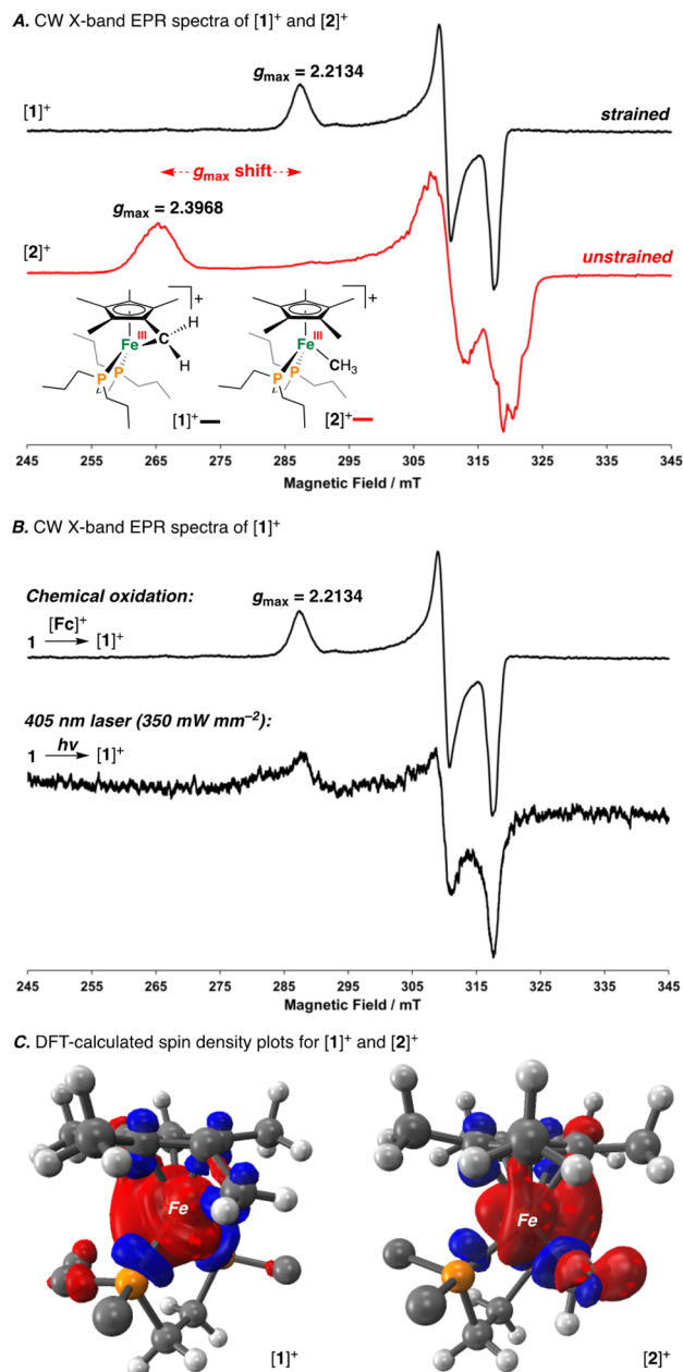
Fig. 5 A) Freeze-quenched CW X-band EPR spectra (8.885 GHz) recorded in 2-MeTHF glass at 77\text{ K} for [1]^+ (black) and [2]^+ (red). (B) Freeze-quenched CW X-band EPR spectra for [1]^+ (top) and a photo-oxidized sample of 1 under 405\text{ nm} ( 350\text{ mW mm}^{-2} ) irradiation (bottom). (C) DFT-calculated spin density plots for [1]^+ and [2]^+ (all C and H atoms from the dnppe ligand, except those C atoms directly attached to P, have been omitted for clarity). \text{Fc} = \text{Cp}_2\text{Fe} .
