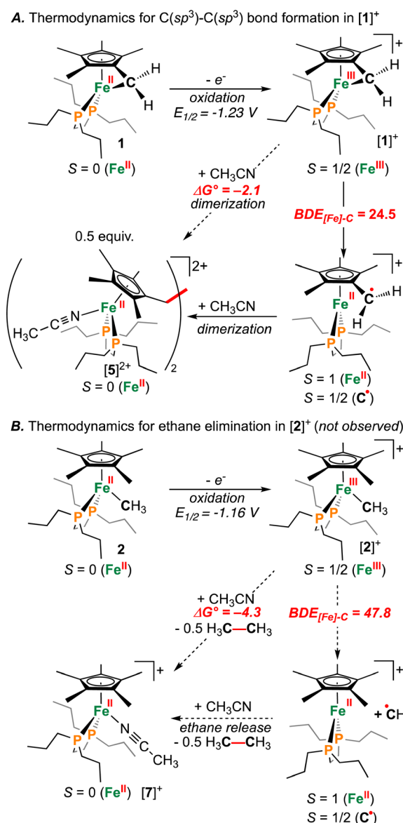
Fig. 7 (A) Thermodynamic calculations showing energies associated with the dimerization of [1]^+ . (B) Analogous calculations for the elimination of ethane ( \text{CH}_3\text{CH}_3 ) from [2]^+ . All energies are in \text{kcal mol}^{-1} .
