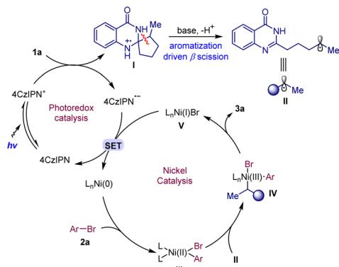
Scheme 4 Proposed Mechanism.
