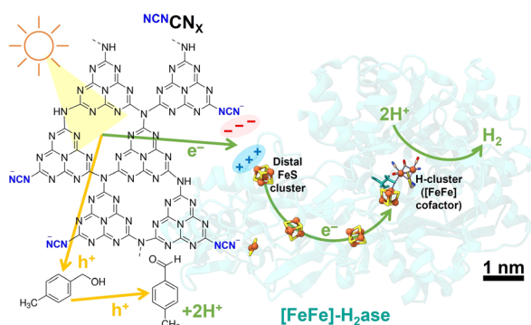
Fig. 1 Schematic of photocatalytic H 2 evolution coupled with alcohol oxidation to aldehyde using an electrostatic NCN CN x /[FeFe]-H 2 ase ( CpI , PDB: 4XDC) assembly. Scale bar refers to enzyme and CN x is not shown to scale.
