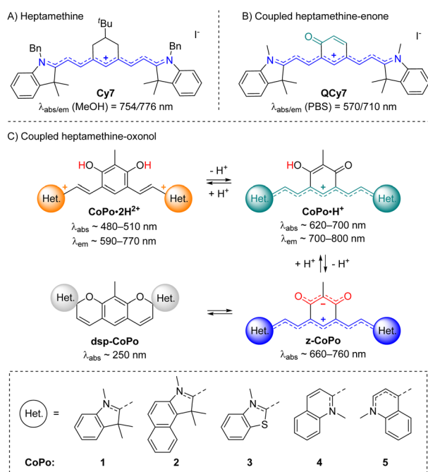
Fig. 2 Previously reported rigidified heptamethine (A) and heptamethine–enone (B) dyes, and coupled heptamethine–oxonol dyes investigated in this work with key optical properties in methanol (C).
