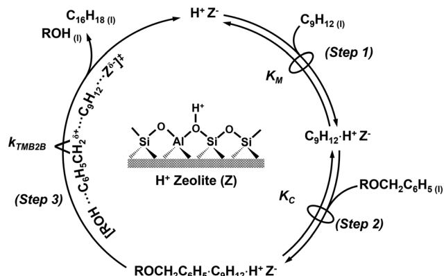
Scheme 2 Proposed reaction mechanism (via the concerted pathway) for benzylation of mesitylene ( C_9H_{12} ) with a benzylating agent ( ROCH_2C_6H_5 ) on a Brønsted acid site ( H^+Z^- ) to form 1,3,5-trimethyl-2-benzylbenzene ( C_{16}H_{18} ) and a leaving group ( ROH ). Steps are described in the text.
