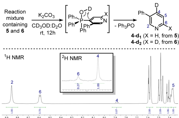
Scheme 4 Deuterodephosphination of the 5/6 mixture (top) and ^1\text{H} NMR and ^2\text{H} NMR spectra ( \text{CDCl}_3 , 400 MHz) of the isolated mixture of 4-d 1 /4-d 2 (bottom). Deuterium incorporation was determined by the relative integration of the signals of hydrogens on the pyridine ring.
