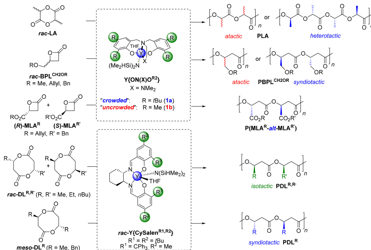
Scheme 1 Examples of yttrium-mediated stereoselective ROP/ROCOP of rac -lactide, rac -4-substituted- \beta -propiolactones, \beta -malolactonates, or rac -dioides. 3,6,9,10
