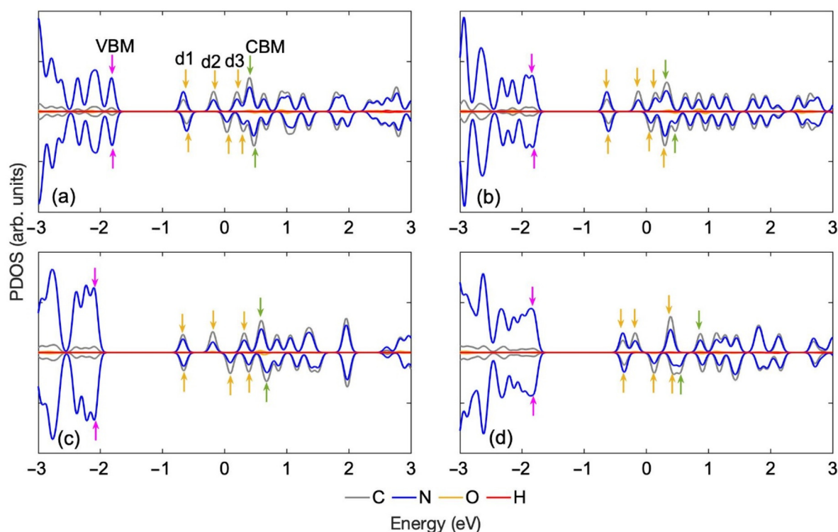
Fig. 2 Partial density of states (PDOS) for the optimized structures of the ON-GCN tautomers shown in Fig. 1: (a) NH-CN, (b) NH 3 , (c) N Hβ and (d) N Hα . Hopping of just one hydrogen leads to substantial changes in the electronic properties. The Fermi level is set to 0 eV. Band edges and defect states are marked with colored arrows: VBM: pink, CBM: green, defects (d1–d3): yellow.
