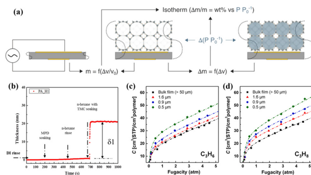
Fig. 6 (a) QCM porosimetry. Reproduced with authorisation from ref. 52 and copyright 2021 by Wiley-VCH GmbH. (b) QCMD thickness–time plots of the thin film composite membrane. Reproduced with authorisation from ref. 63 and copyright 2017 by Elsevier. Sorption isotherms of (c) C_3H_6 and (d) C_3H_8 for 6FDA-DAM thin films with varying thicknesses determined by the QCM. Reproduced with authorisation from ref. 64 and copyright 2022 by Elsevier.
