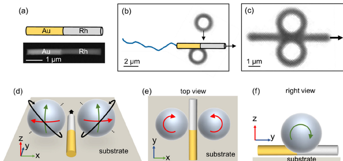
Fig. 1 Au–Rh nanorod motors collect and spin tracer microspheres. (a) Backscattered SEM image of an Au–Rh nanorod and its cartoon diagram. (b and c) Two \text{SiO}_2 microspheres 2 \mu\text{m} in diameter and zeta potential of -46 mV are attracted by a moving Au–Rh nanorod (b) and collected to the metal junction of the rod (c), in 5 wt% \text{H}_2\text{O}_2 . (d) Schematic of the tracer microspheres on either side of a Au–Rh nanorod. Tracers spin about a tilted axis (dashed black lines) vertical to the long axis of the rod motor. The 3D spinning (black arrows) can be considered as a combination of spinning on the xy plane (e, red arrows) and spinning on the yz plane (f, green arrows). The exposure of optical micrographs in (b) and (c) has been greatly increased (to the point of overexposure) to improve the contrast without losing the microscopic detail or distorting the image. The same modification was applied to other optical micrographs in this article.
