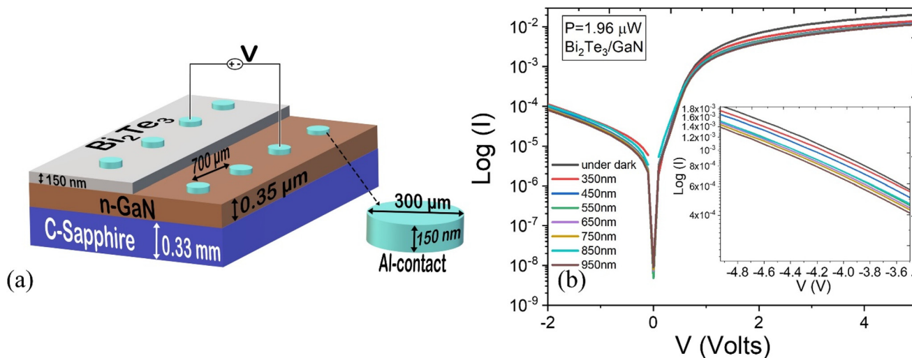
Fig. 1 (a) Schematic of the device structure of \text{Bi}_2\text{Te}_3/\text{n-GaN/S} . (b) Plot of the semi-log ( I - V ) characteristics for the \text{Bi}_2\text{Te}_3/\text{n-GaN} heterostructure device under dark and illumination conditions when the wavelength of the irradiating wavelength of the light was varied from 350 nm to 950 nm at a constant incident light power of 1.96 \mu\text{W} ; inset shows the reverse saturation current in the reverse bias ( V = -4.8 \text{ V} to -3.6 \text{ V} ).
