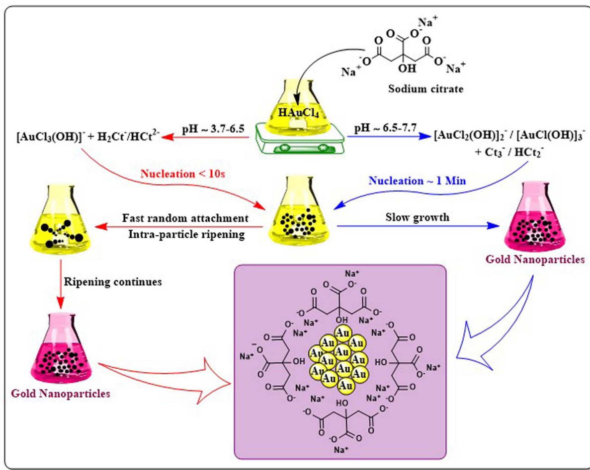
Fig. 4 Turkevich's method for AuNP synthesis and the reaction route according to different pH systems. In acidic pH conditions, nucleation is fast ( < 10 \text{ s} ) with random particle attachment followed by ripening, whereas a slightly basic pH directs slow nucleation ( \sim 1 \text{ min} ), followed by slow growth of intermediate particles to synthesise gold nanoparticles.
