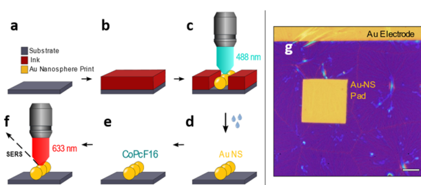
Fig. 1 Laser-induced printing of Au nanospheres on a surface of choice. (a–f) Scheme for printing of a ready-to-measure SERS substrate. (a and b) Spin-coating of a thin film of the ink solution onto the substrate surface. (c) Selective printing of an Au-NS structure by raster scanning the sample through the focused laser beam, causing the Au 32 nanocluster to coalesce to Au-NS. (d) Lift-off: wet removal of the unexposed ink film leaves a clean surface with the Au-NS pattern on top. (e) Uniform thin layer deposition of CoPcF 16 on the substrate. (f) Detecting SERS of the CoPcF 16 molecule on top of the Au-NS pattern. (g) Optical micrograph of a printed rectangular Au-NS pad (scale bar 10 \mu\text{m} ).
