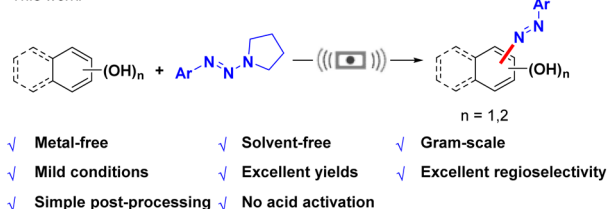
Scheme 1 General synthetic pathway for azo dyes.
