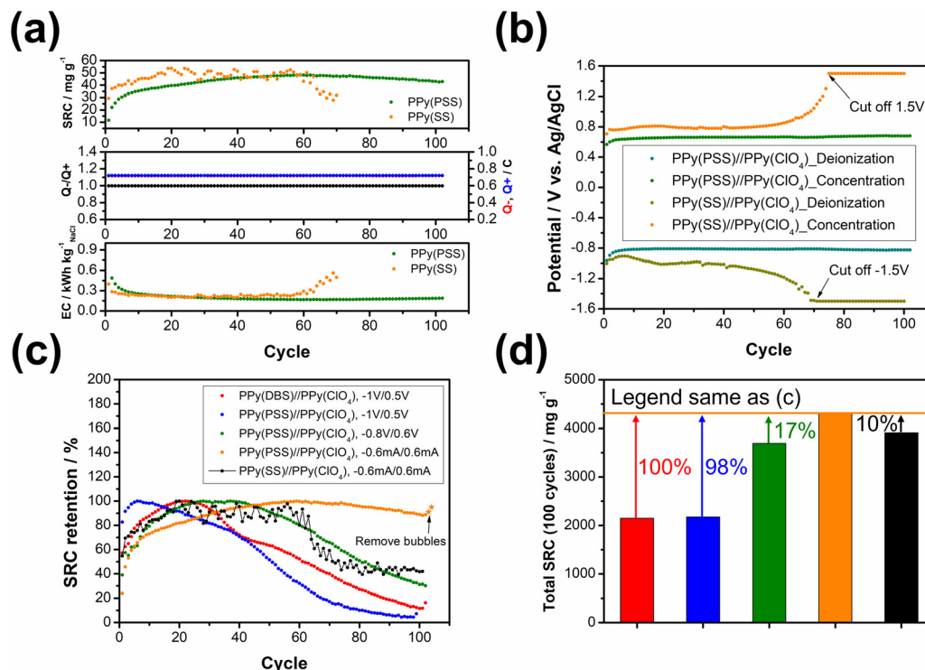
Fig. 5 (a) Comparisons between the salt removal capacity (SRC) profile, Q^+/Q^- value, and energy consumption (EC) profile for PPy(PSS)//PPy( \text{ClO}_4 ) and PPy(SS)//PPy( \text{ClO}_4 ) with deionization, concentration = -0.6\text{ mA}/0.6\text{ mA} , 20 min/20 min. (b) The potential profile during the operation in (a). (c) The retention comparison of all systems. (d) Accumulated SRC after 100 cycles for all systems.
