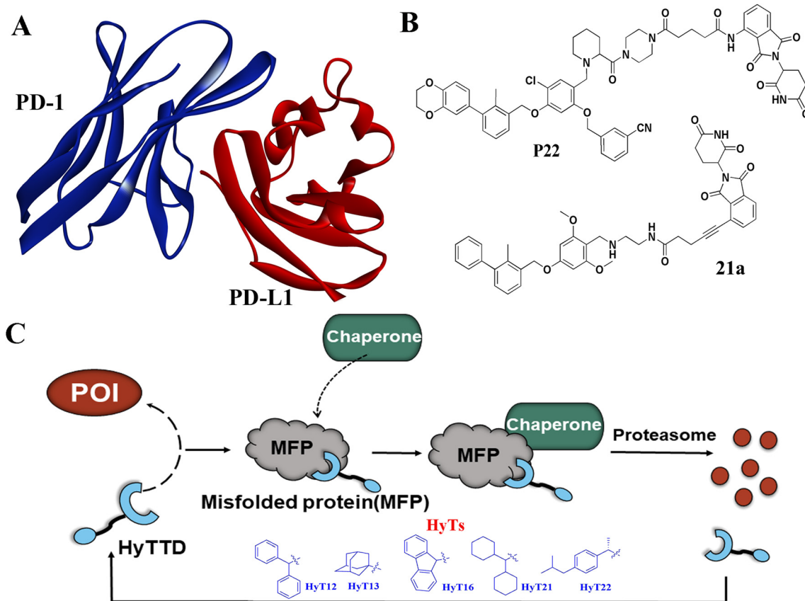
Fig. 1 The strategies to develop PD-L1 degraders. A) The complex of PD-1 and PD-L1 (PDB-ID:4ZQK); B) the PD-L1 degraders linked with the cereblon ligand; C) the proposed mechanism for HyTDD to degrade the targeted protein.
