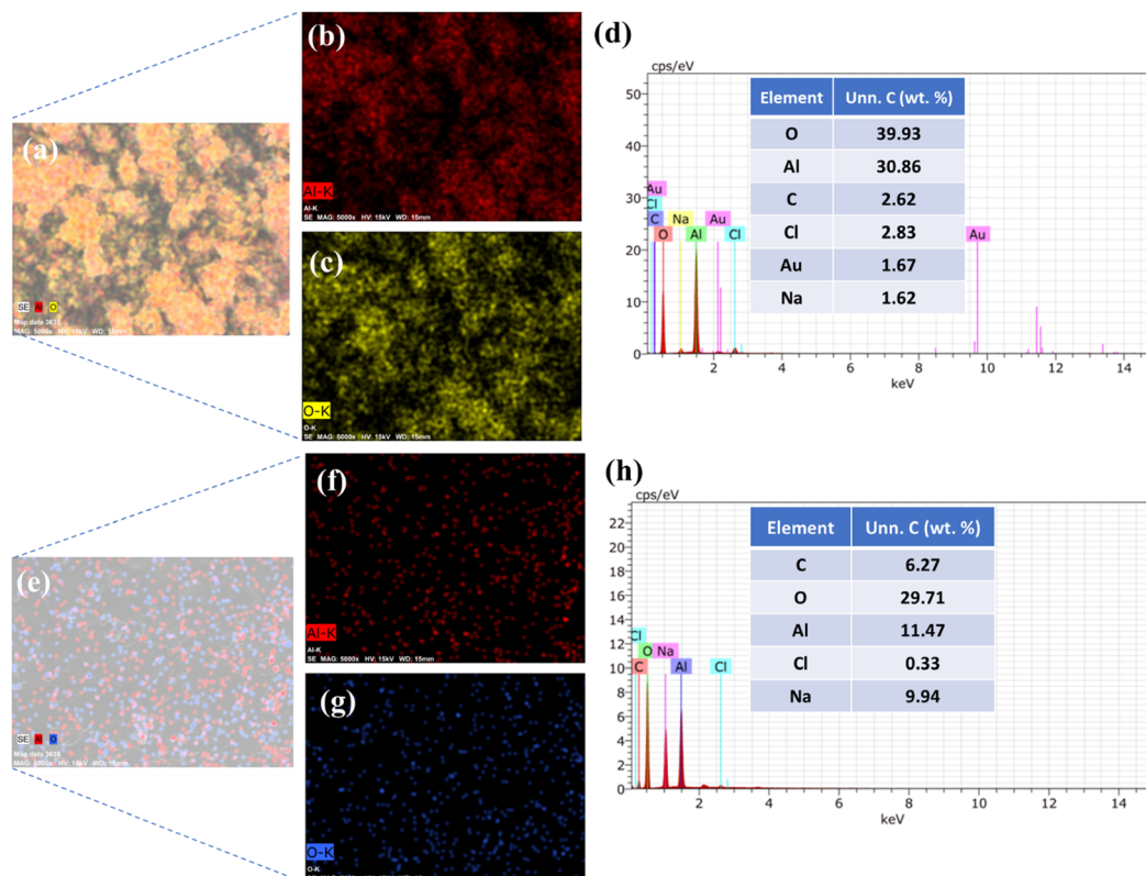
Fig. 4 Mapping of \text{Al}_2\text{O}_3 (a)–(c) and EDX of \text{Al}_2\text{O}_3 (d). Mapping of ALOOH (e)–(g) and EDX of ALOOH (h).
