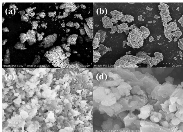
Fig. 3 FE-SEM of \text{Al}_2\text{O}_3 (a) and (b) particles at scales of 40.0 \mu\text{m} and 20.0 \mu\text{m} , respectively. FESEM of ALOOH (c) and (d) particles at scales of 4.0 \mu\text{m} and 1.0 \mu\text{m} , respectively.
