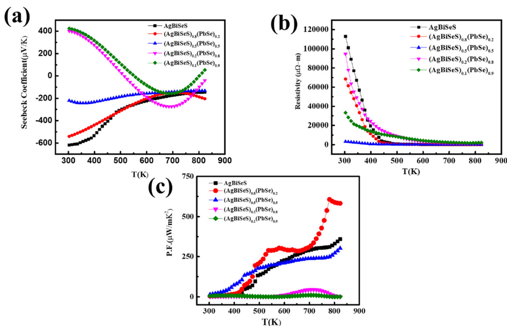
Fig. 4 Temperature-dependent (a) Seebeck coefficient; (b) electrical resistivity and (c) power factor of the alloy system (\text{AgBiSeS})_{1-x}(\text{PbSe})_x .
