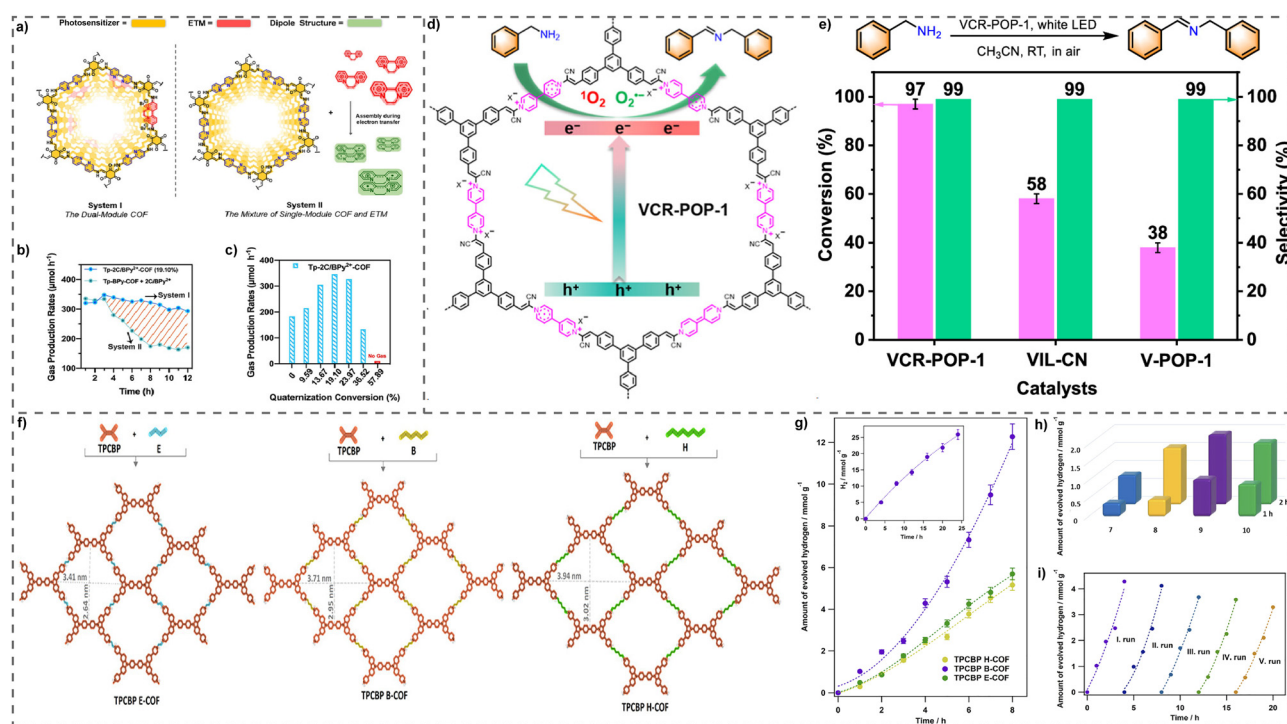
Fig. 11 (a) Schematic diagram of the dual-module COF (System I) and the mixture of single-module COF with unembedded ETM (System II). (b) The hydrogen evolution test of the integrated Tp-2C/ByPy 2+ -COF (19.10%) and the bare Tp-BPy-COF mixed with additional 2C/ByPy 2+ used as an ETM under visible-light irradiation. The orange integral area roughly reflects the hydrogen evolution difference between the two photocatalytic systems. (c) HERs of Tp-2CPBy 2+ -COF (10 mg) with different quaternization conversions. Reproduced with permission from ref. 107. Copyright 2022 Wiley-VCH. (d) Schematic representation of photocatalytic oxidative coupling of benzylamine through VCR-POP-1. (e) Photocatalytic performance in white-light-driven photocatalytic oxidative coupling of benzylamine into imine over different catalysts VCR-POP-1, VIL-CN, and V-POP-1. Reproduced with permission from ref. 110. Copyright 2022, American Chemical Society. (f) Schematic representation of TPCBP X-COF [X = ethyl (E), butyl (B), and hexyl (H)] structures. (g) Photocatalytic hydrogen evolution activities of TPCBP X-COFs. (h) pH effect of TEOA. (i) Photocatalytic stability test of TPCBP X-COFs. Reproduced with permission from ref. 108. Copyright 2022, American Chemical Society.
