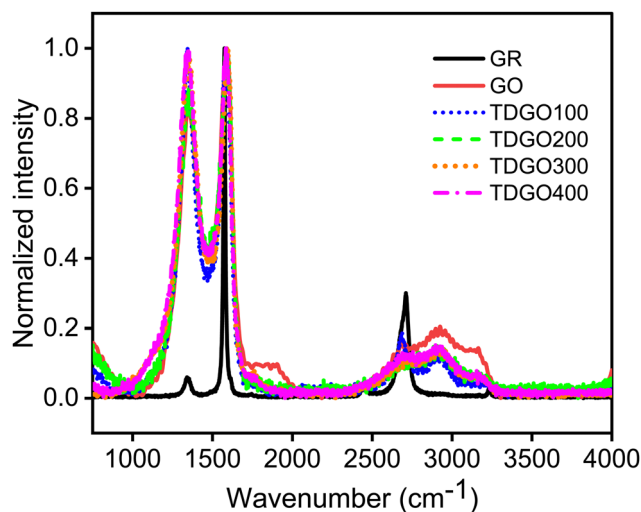
Fig. 2 Raman spectral analysis of graphite (GR), graphite oxide (GO), and TDGO100, TDGO200, TDGO300 and TDGO400 active materials.
