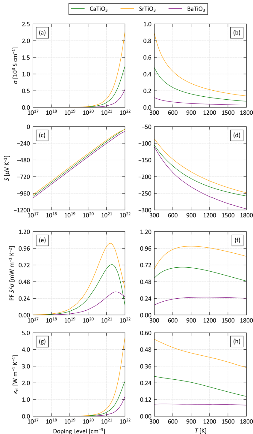
Fig. 4 Comparison of the calculated averaged electrical conductivity \sigma (a)/(b), Seebeck coefficient S (c)/(d), power factor S^2 \sigma (PF) (e)/(f) and electronic thermal conductivity \kappa_{\text{el}} (g)/(h) of the three structures examined in this work as a function of doping level at a fixed T = 1000 K (a)/(c)/(e)/(g) and as a function of temperature at a fixed doping level n = 10^{21} cm -3 (b)/(d)/(f)/(h).
