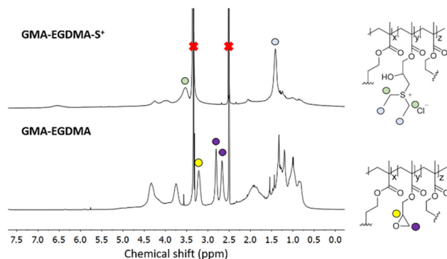
Fig. 3 ^1\text{H} NMR spectrum in DMSO- D_6 (residual solvent signals are labelled with red crosses) of GMA-EGDMA- S^+ , with characteristic signals of the sulfonium group at \delta = 1.4 ppm labelled blue and at \delta = 3.5 ppm labelled green.
