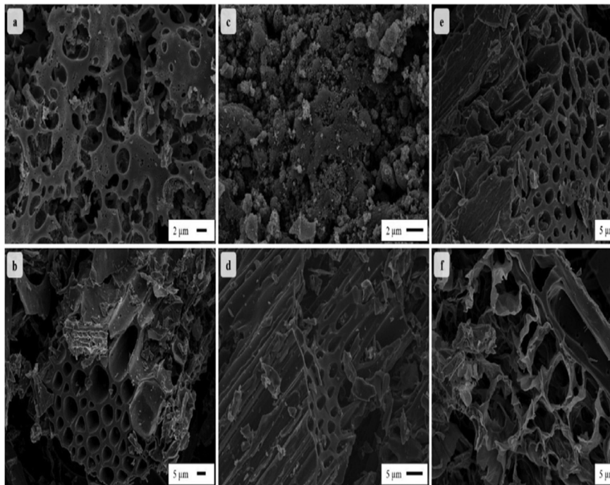
Fig. 19 SEM microstructures of the activated carbons: a) KOH-K, b) KOH-KB, c) \text{H}_3\text{PO}_4\text{-K} , d) \text{H}_3\text{PO}_4\text{-KB} , e) \text{MnO}_2/\text{KOH-KB} , and f) \text{MnO}_2/\text{H}_3\text{PO}_4\text{-KB} . Reproduced from ref. 162 with permission from Elsevier, copyright 2020.
