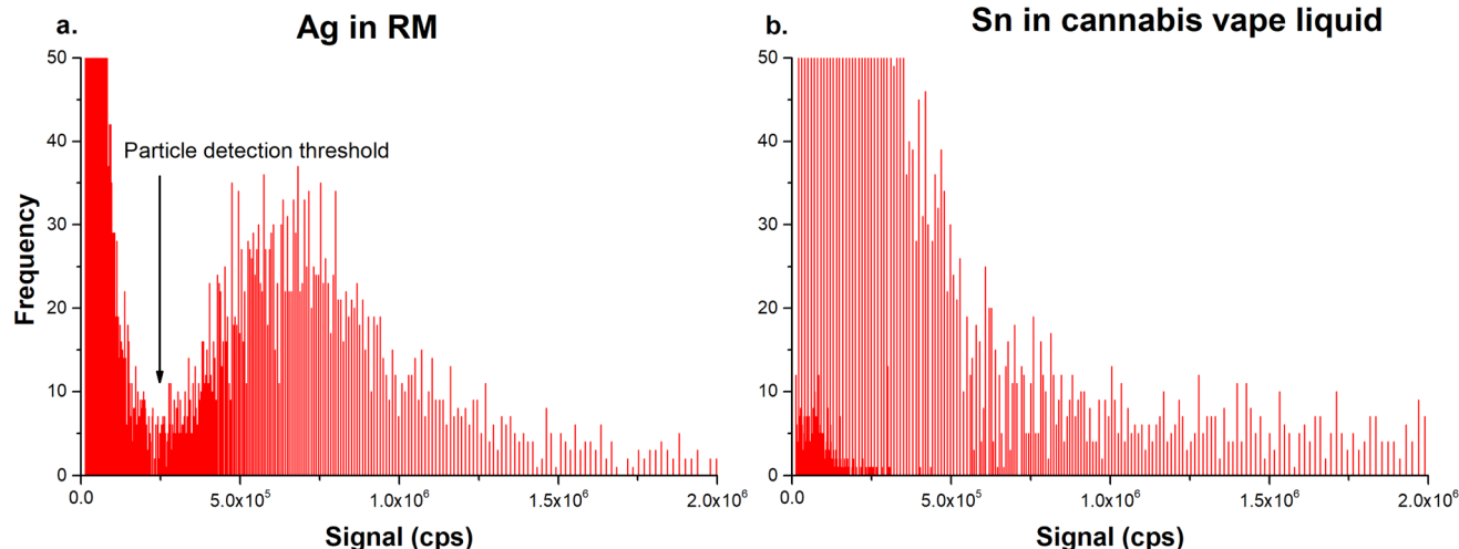
Fig. 3 Signal distribution of (a) 2837 Ag NPs in 60 nm RM, and (b) 2487 Sn NPs in cannabis vape liquid. Particle detection threshold distinguishes between signal generated by dissolved ions and NPs of a given analyte.
