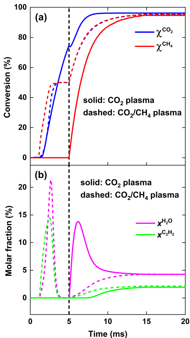
Fig. 9 \text{CO}_2 and \text{CH}_4 conversion (a), as well as \text{H}_2\text{O} and \text{C}_2\text{H}_2 molar fraction (b), as a function of time, for \text{SEI} = 220 \text{ kJ mol}^{-1} . The solid and dashed lines indicate the results for the \text{CO}_2 plasma with post-plasma \text{CH}_4 injection, and for the \text{CO}_2/\text{CH}_4 plasma with post-plasma \text{CO}_2/\text{CH}_4 injection, respectively. The vertical dashed line at 5 ms indicates the post-plasma mixing.
