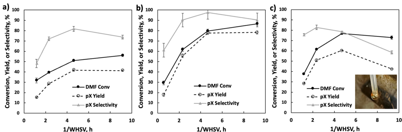
Fig. 5 Reactor performance at various 1/WH SVs at 350 °C (1.15 h, 2.31 h, 4.61 h, and 9.15 h, panel a), 375 °C (0.57 h, 2.33 h, 4.66 h, and 9.24 h, panel b), and 400 °C (1.18 h, 2.35 h, 4.70 h, and 9.33 h, panel c). Conditions: 750 psig back pressure, 0.5 g P-BEA(25), 20 wt% DMF feed; 0.025 mL min -1 liquid flow rate.
