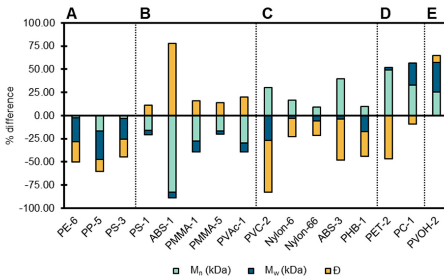
Fig. 10 Percent difference of number-average molecular mass ( M_n ), weight-average molecular mass ( M_w ), and dispersity ( \mathcal{D} ) after cryomilling. Increasing % difference indicates an increase following cryomilling, and polymers shown exhibit differences of >15\% in at least one category. (A) M_n , M_w , and \mathcal{D} all decrease for PE-6, PP-5, and PS-3. (B) M_n and M_w decrease, and \mathcal{D} increases for PS-1, ABS-1, PMMA-1, PMMA-5, and PVAc-1. (C) M_w and \mathcal{D} decrease, and M_n increases for PVC-2, nylon-6, nylon-66, ABS-3, and PHB-1. (D) \mathcal{D} decrease, M_n and M_w increases for PET-2, and PC-1. (E) M_n , M_w , and \mathcal{D} all increase for PVOH-2. M_n represents the most abundant, often lower, molecular masses, whereas M_w represents the higher molar mass portion of the bulk polymer. A decrease in M_n , M_w , and \mathcal{D} indicates both a decrease in low and high molecular mass components and distribution of masses.
